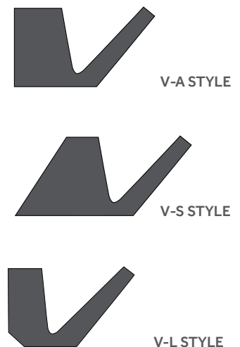
Figure 1.1 Standard V-ring shapes available
