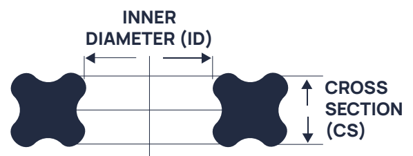
Figure 1.1 Quad-ring® measurements
